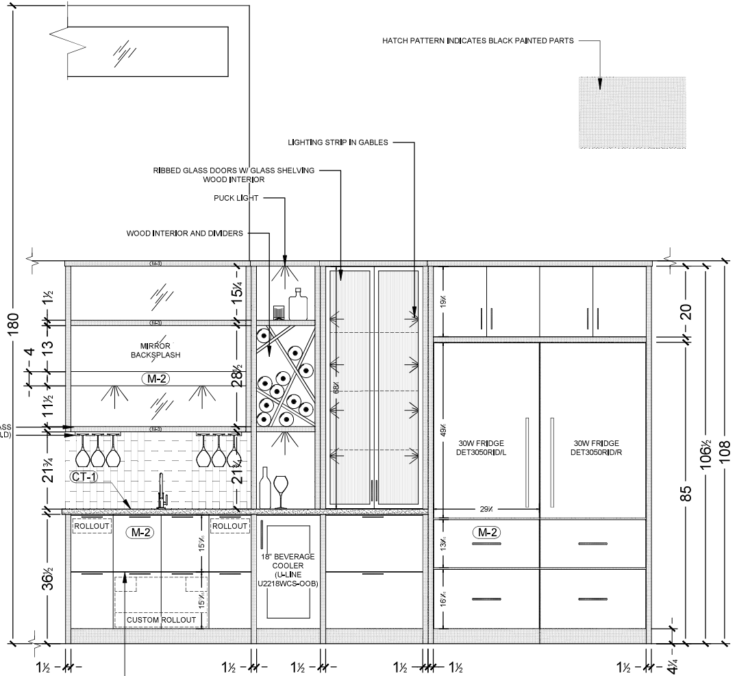
KITCHEN ELEVATION
