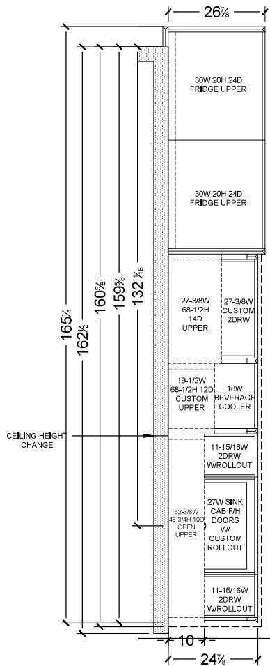
KITCHEN LAYOUT
