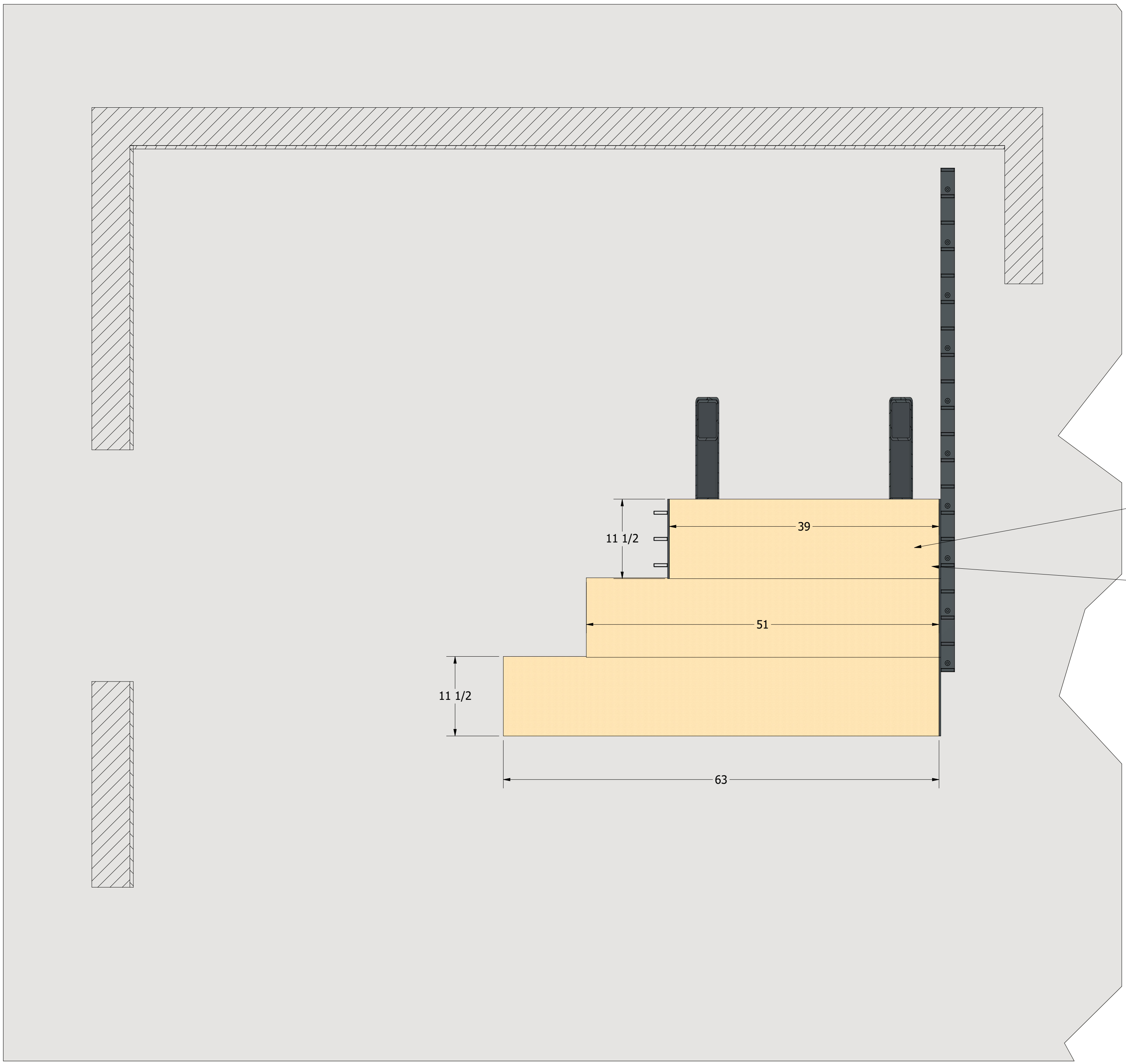
SECTION A-A SCALE .1
