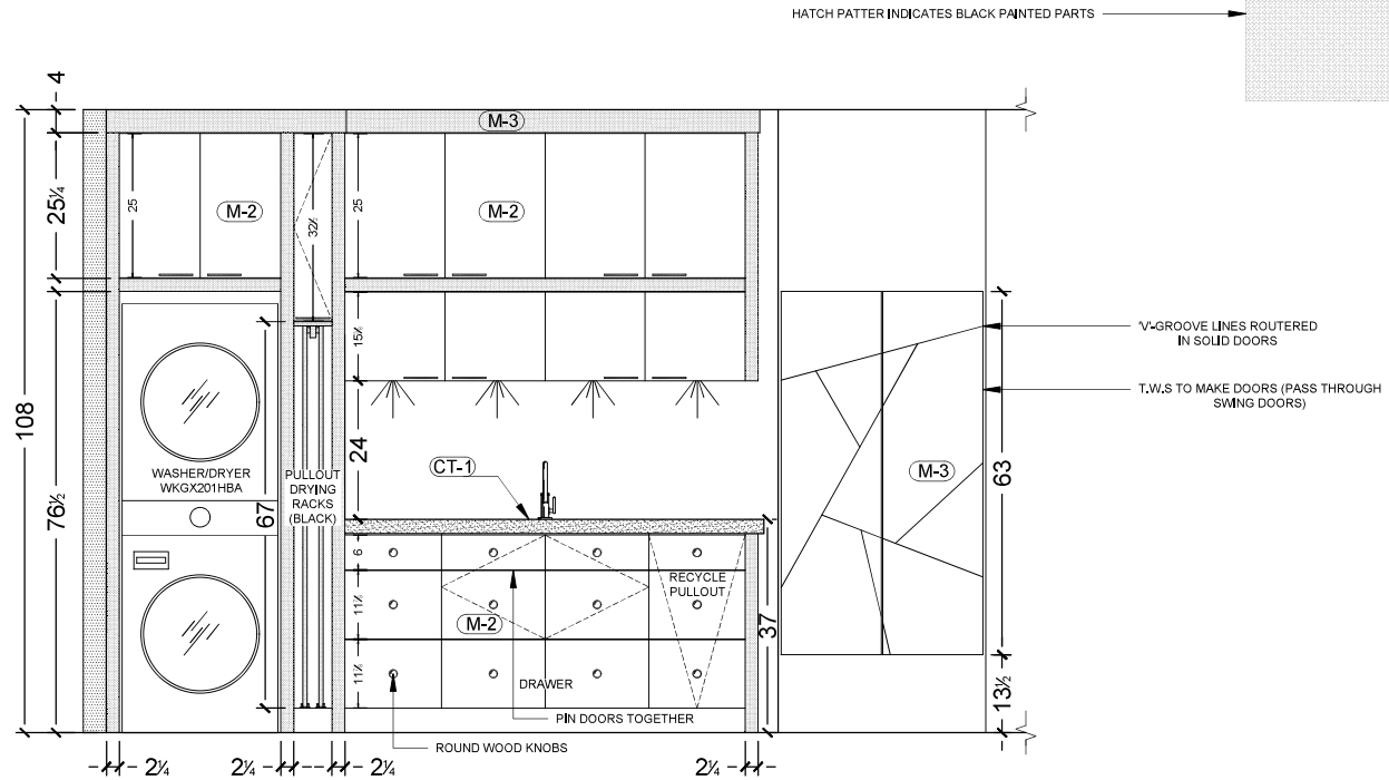
1 LAUNDRY ELEVATION SCALE: 1/2" = 1'0"
