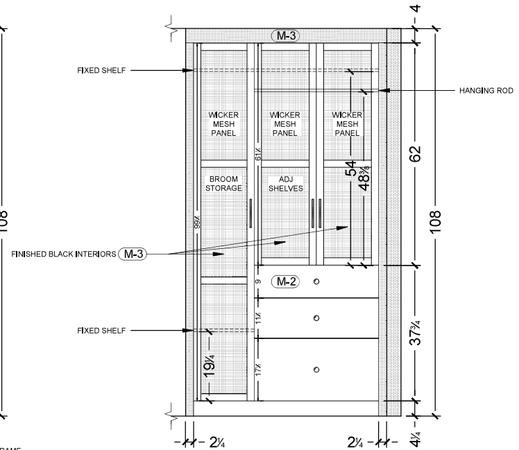
2 LAUNDRY ELEVATION SCALE: 1/2" = 1'0"
