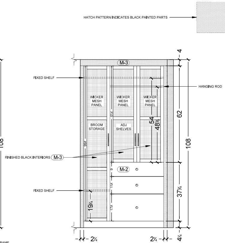
2 LAUNDRY ELEVATION SCALE: 1/2" = 1'0"
