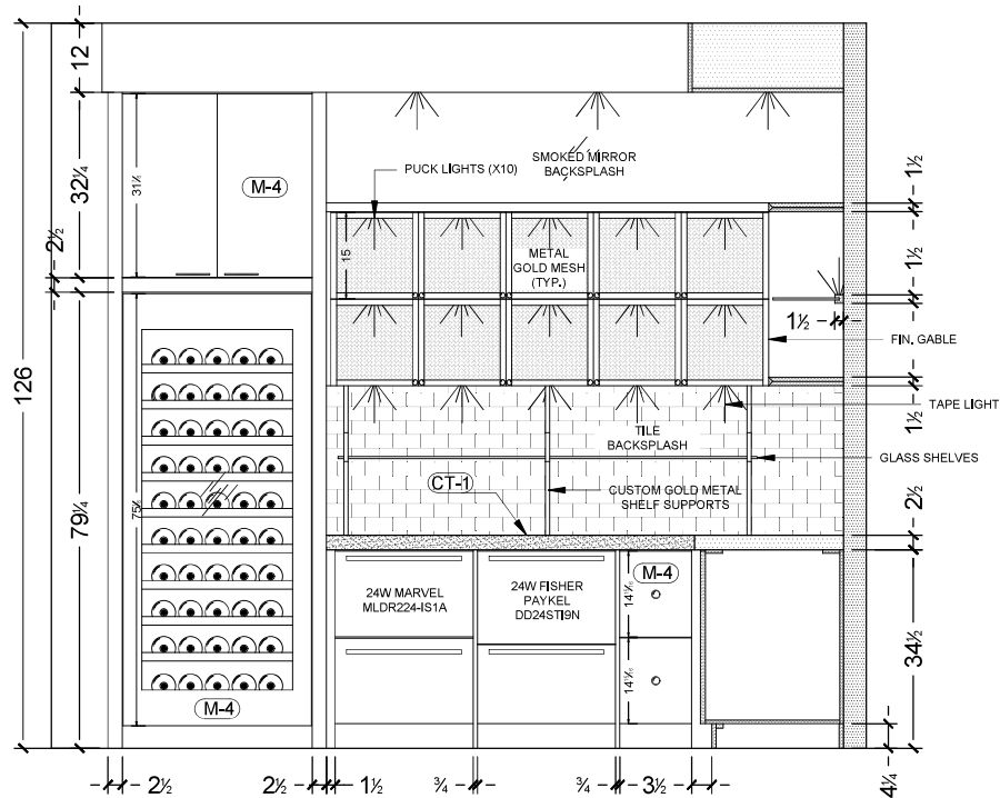
1 GAMES ROOM ELEVATION SCALE: 1/2" = 1'0"
