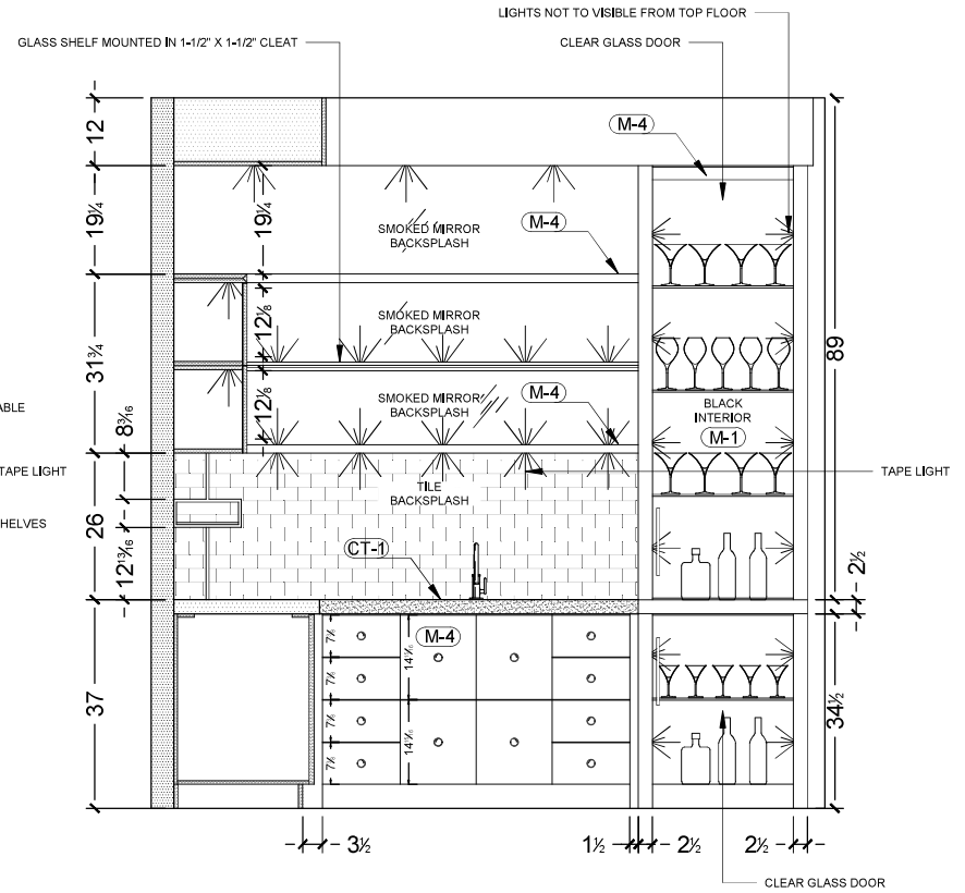
2 GAMES ROOM ELEVATION SCALE: 1/2" = 1'0"
