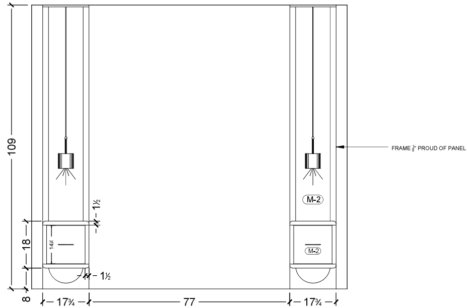
1 PRIMARY BEDROOM NIGHTSTANDS SCALE: 1/2" = 1'0"
