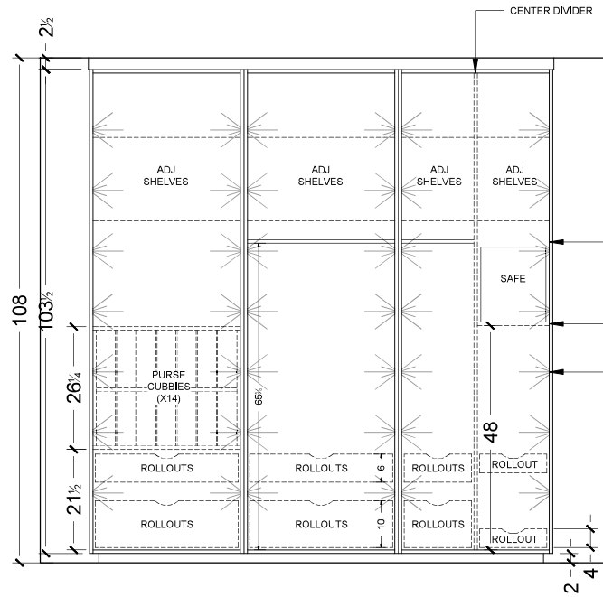
1 PRIMARY CLOSET W/O DOORS SCALE: 1/2" = 1'0"
