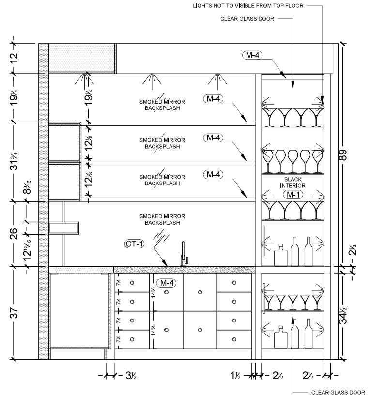
2 GAMES ROOM ELEVATION SCALE: 1/2" = 10"
