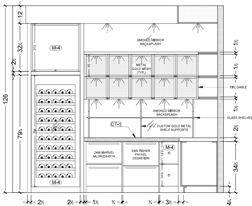
1 GAMES ROOM ELEVATION SCALE: 1/2" = 10"
